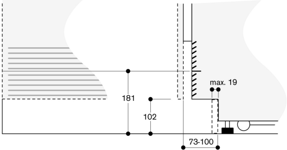
Base detail
