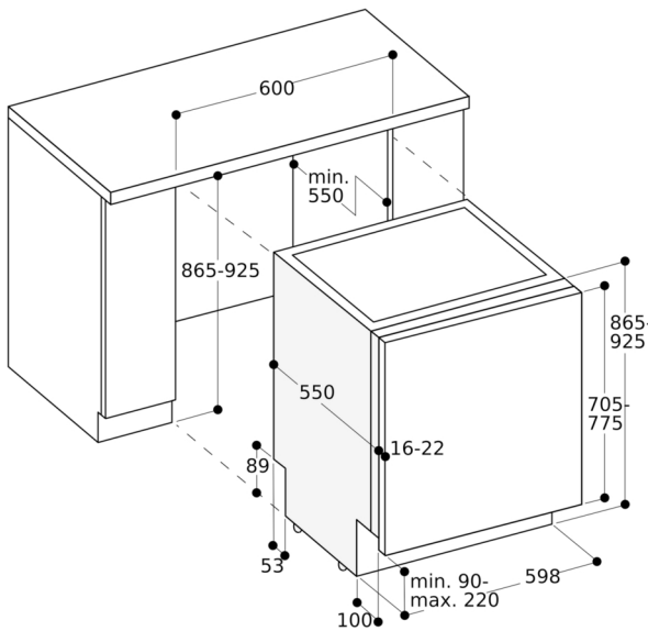
86.5 cm high dishwasher
