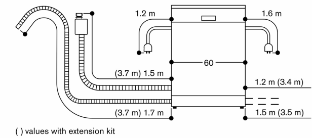
Connection dimensions for a 60 cm wide dishwasher
