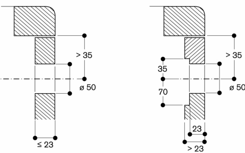
Installation of the control knob; surface mounting
